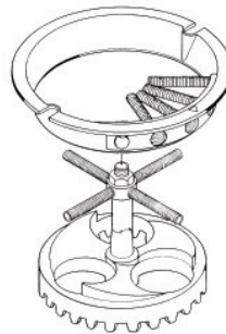
B10 - Capsule Toy Conversion 1 1/2" dia. / 39mm holes with heavy duty agitator & 4 silver housing springs Use - Capsule products 1", 1 1/8", 1.3" round or acorn shaped
