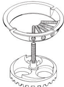
B8 - Capsule Gum Conversion 1 1/2" dia. / 38mm holes with silver springs Use - Gumballs 1 3/16" - 1 3/8" dia. / 30-35mm 250-900 count
