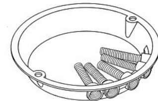
B6 - Deep Adjustable Anti-Milking Conversion For extra large portions With silver springs (hard products) With black spring (soft products) Use - nuts, confections, chicklets, animal feed, mike & ikes, jelly beans
